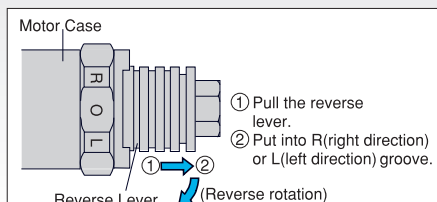
How to reverse the rotation with YD-3,3A, YD-4,4A, YD-5A.
